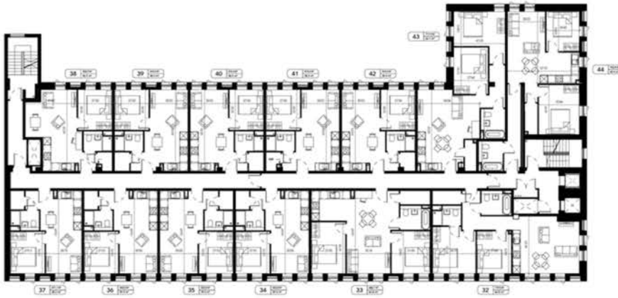
THIRD FLOOR
